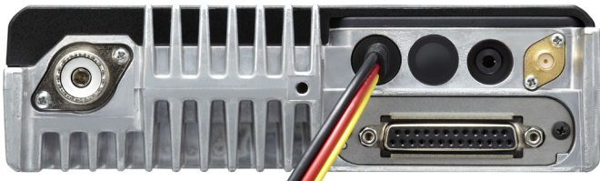
Rear Panel VM5000/6000
